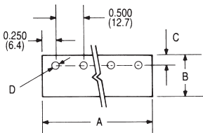
DUAL TO-220
