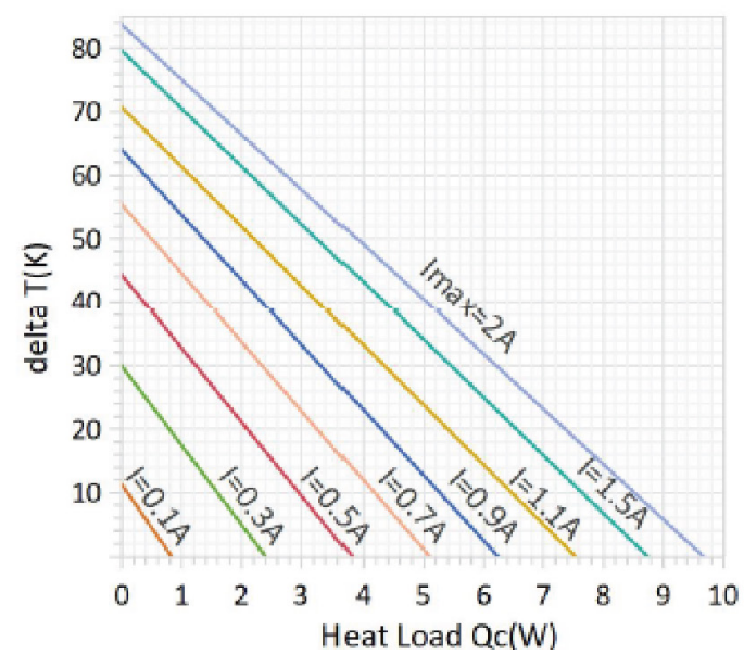
\Delta T vs. Heat Load
