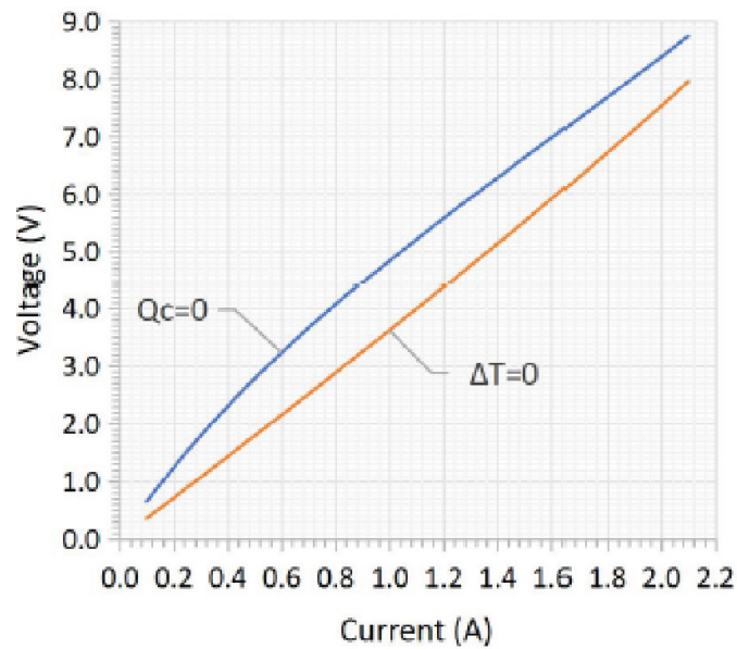
Voltage vs. Current
