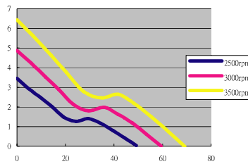
9238 PQ CURVE
