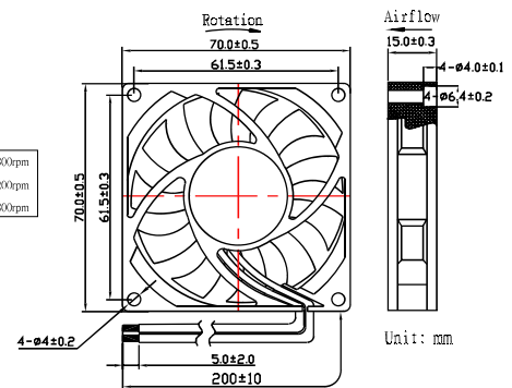
DIMENSIONS DRAWING
