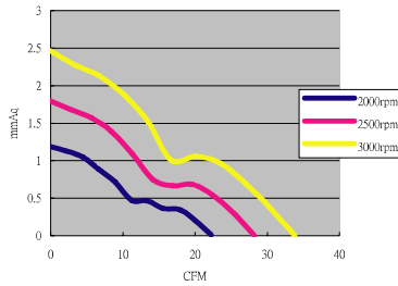
8020 PQ CURVES
