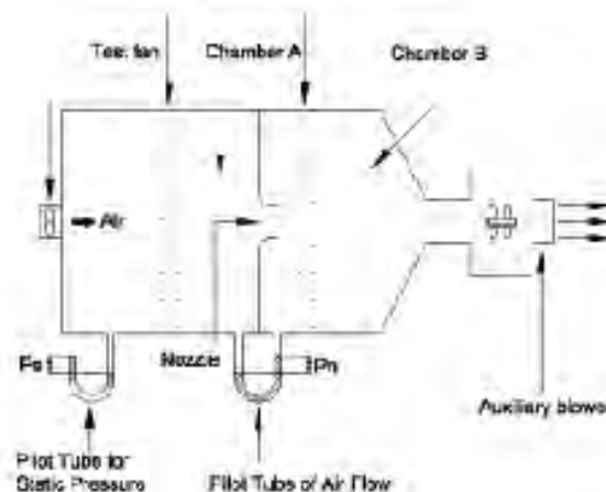
The Measuring Method-double Chamber
