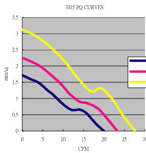
P&Q CURVE
